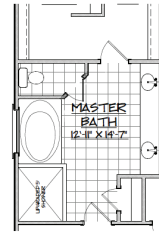
OPTIONAL MASTER BATHROOM WITH 5' SHOWER & EXTENDED VANITY
